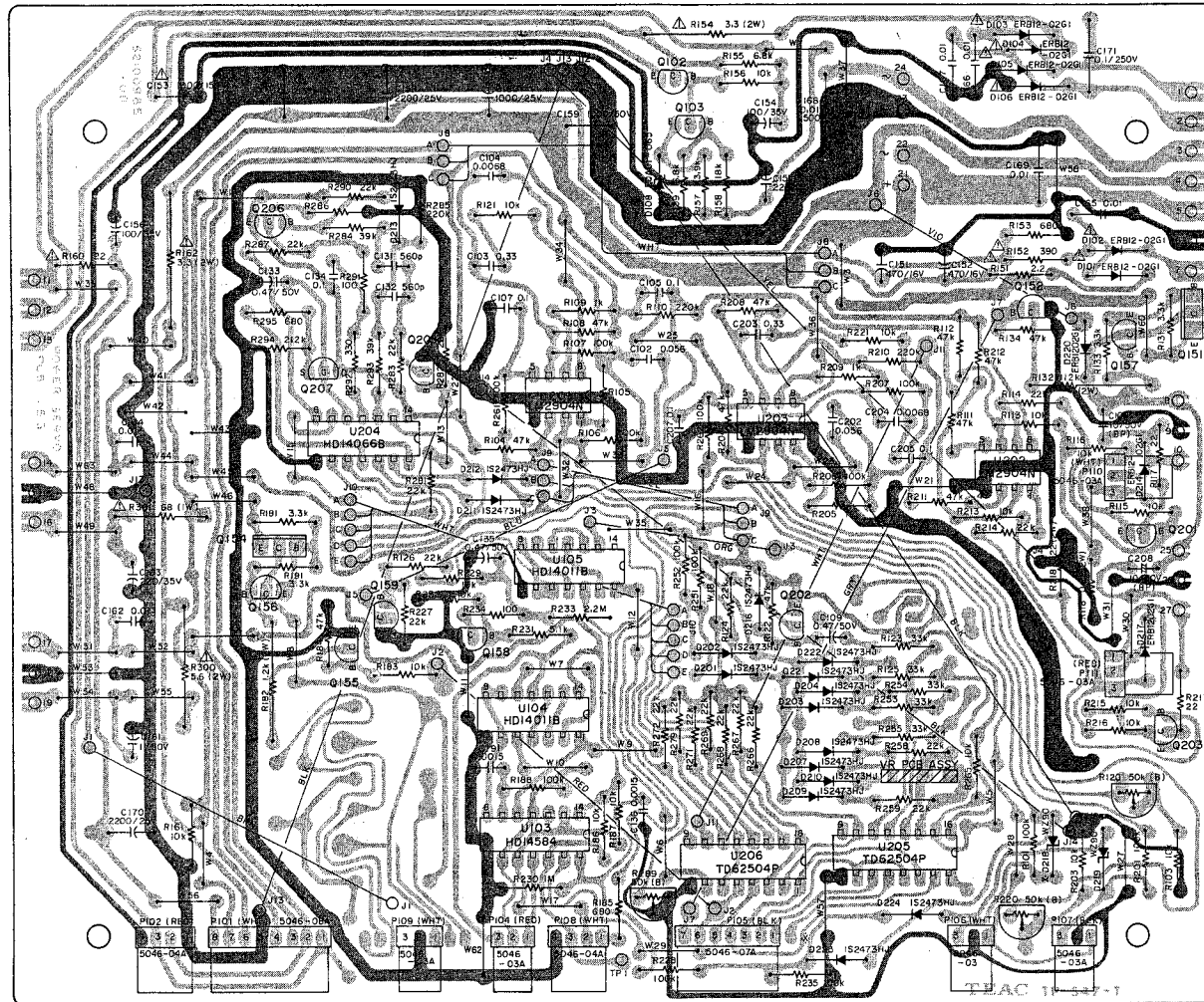
POWER/SERVO PCB ASSY
