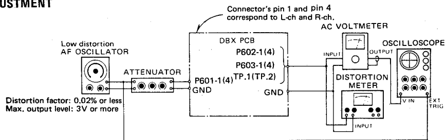
Fig. 3-13 Decoder adjustment setup
