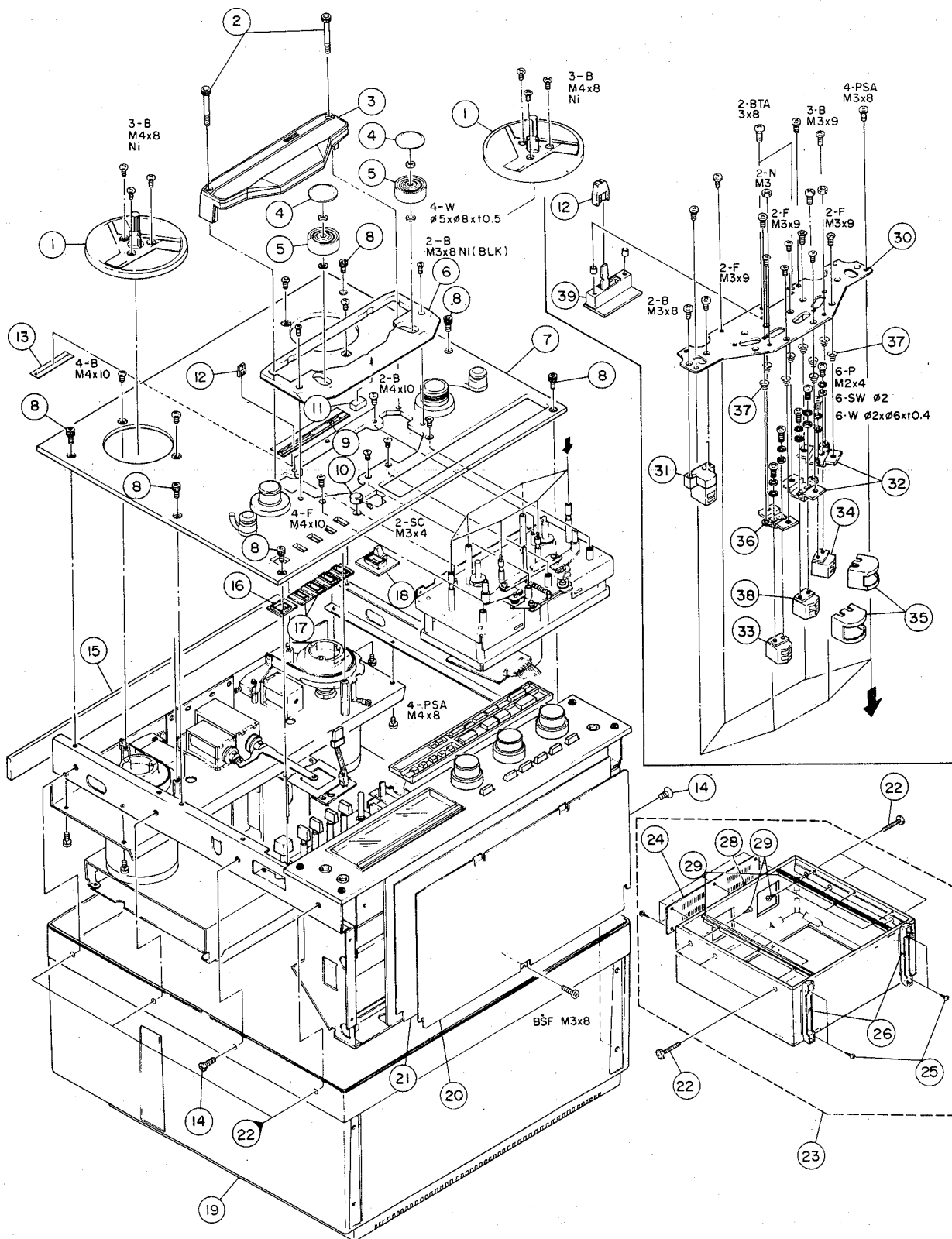
EXPLODED VIEW -1 (X-1000M)
