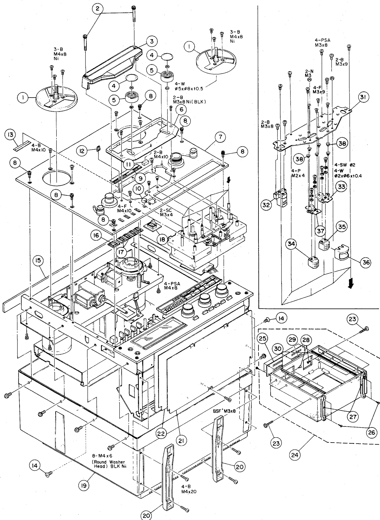
EXPLODED VIEW -2 (X-1000)
